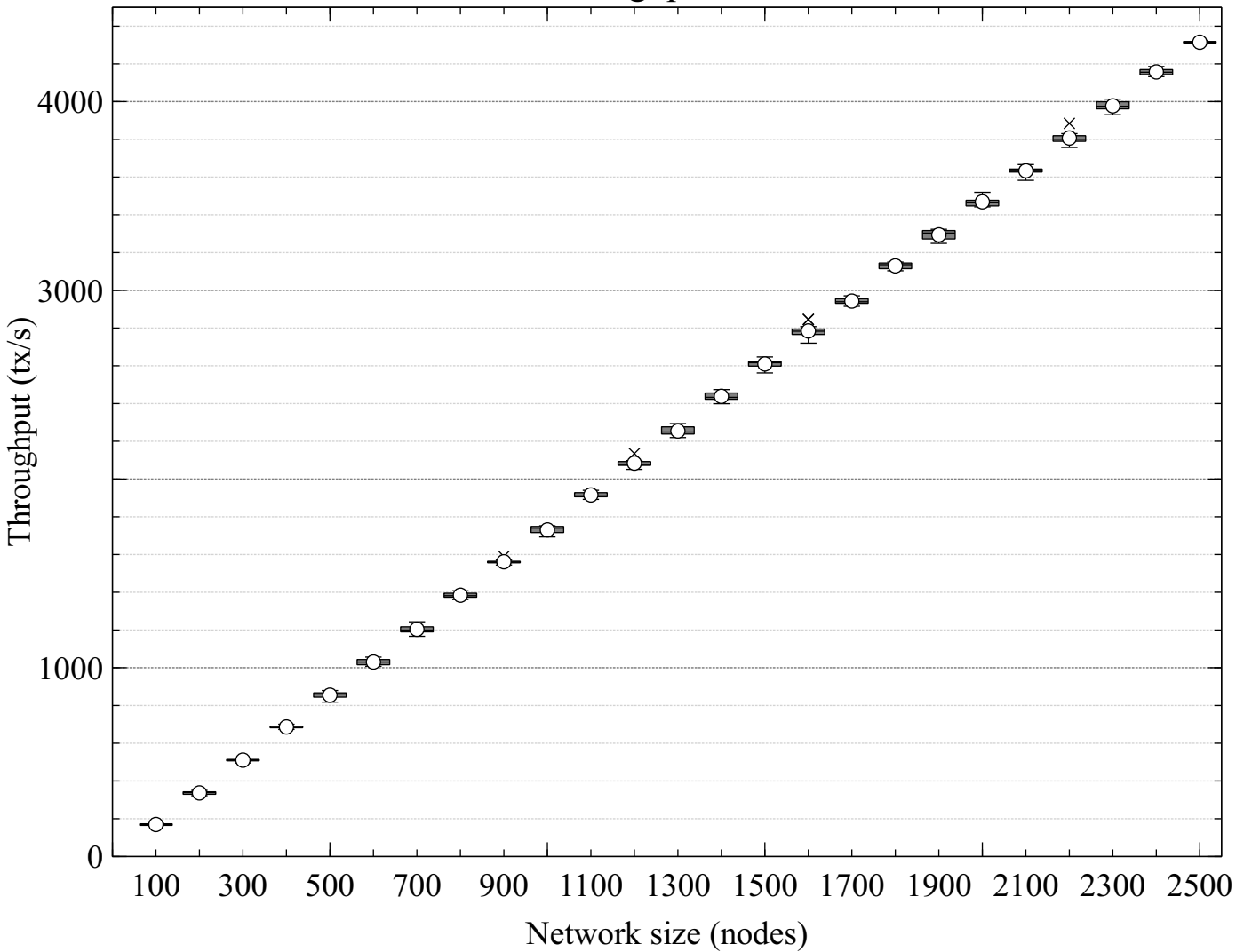
Transaction throughput vs. Network Size
