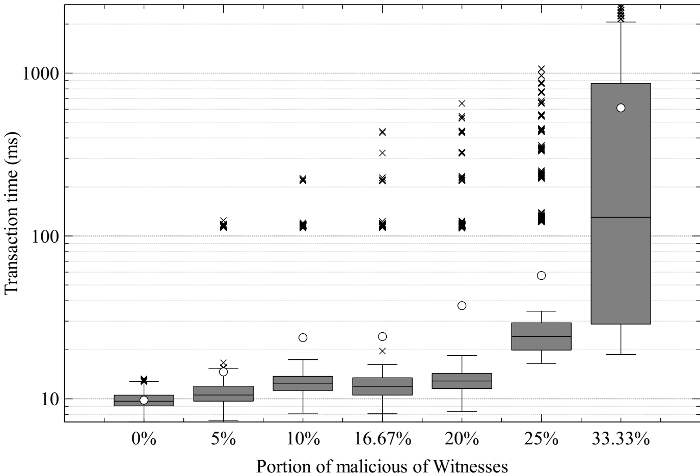
Transaction Time vs. Portion of malicious nodes
