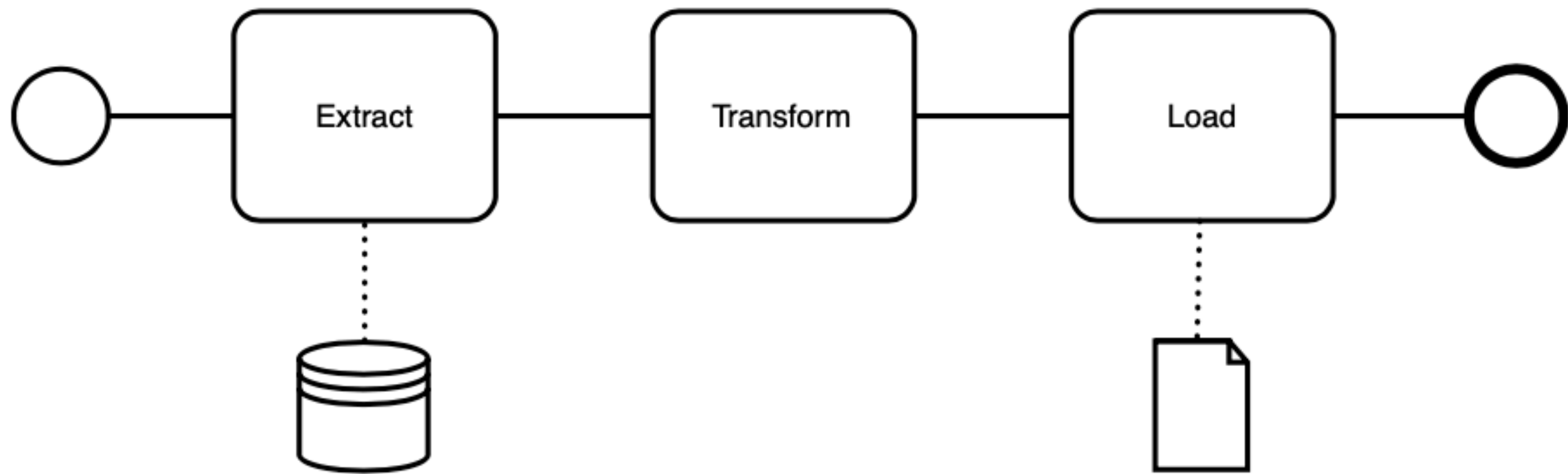
Figure 4. BPMN example
